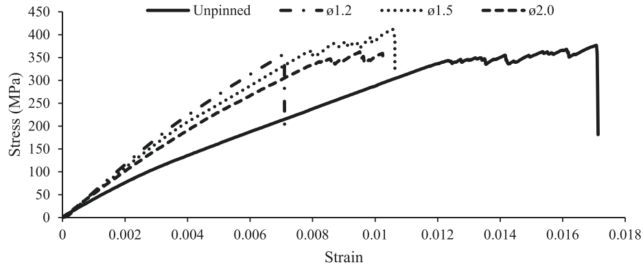
Fig. 3. Typical tensile stress versus strain curves for unpinned and pinned samples.
