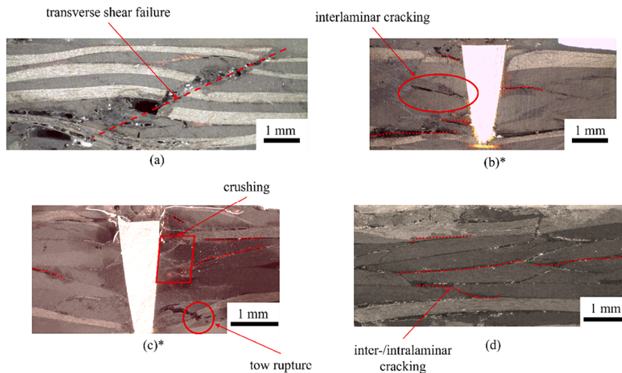
Fig. 6. Micrographs showing compressive failure mechanics in (a) unpinned, (b) pin location in ø1.2, (c) pin location in ø2.0, and (d) away from the pin in ø2.0 specimens.
