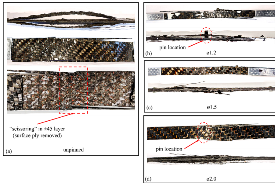
Fig. 5. Fractured tensile specimens showing (a) unpinned, (b) ø1.2, (c) ø1.5, and (d) ø2.0.
