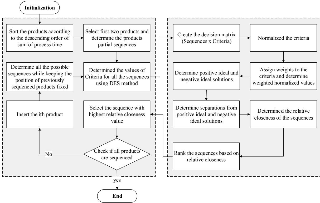
Figure 2 Flowchart of proposed Smart Multi-Criteria Nawaz, Enscore, and Ham (SMC-NEH) algorithm
