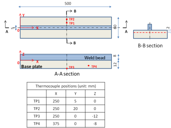
Fig. 2: Geometry of the WAALM sample.
