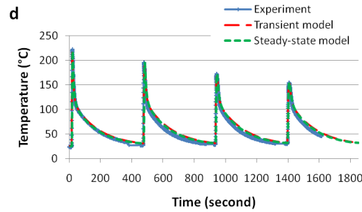
Fig. 6: Temperature verification on the measuring positions of (a) TP1 (250, 5, 0), (b) TP2 (250, 20, 0), (c) TP3 (250, 0, -12), (d) TP4 (375, 0, -8).
