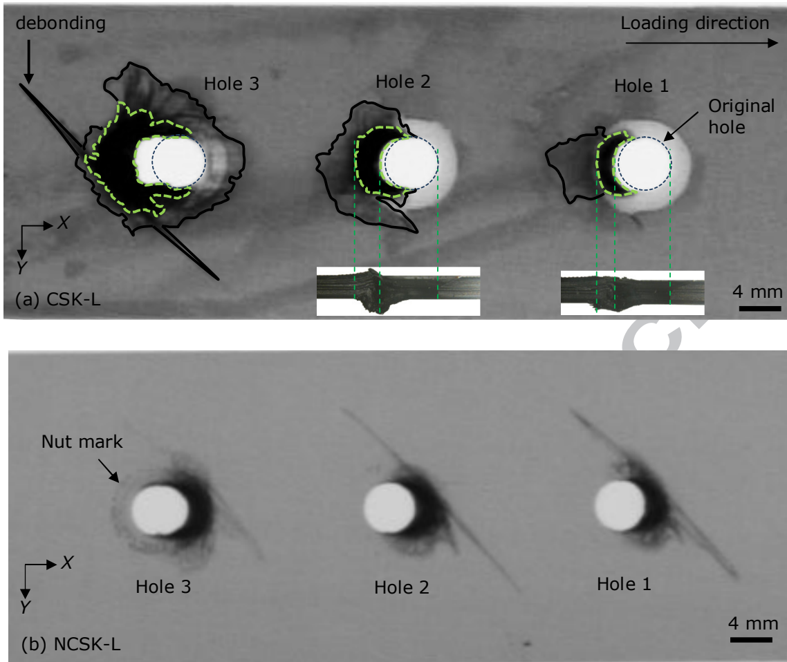
Figure 9: X-ray image of three-bolt CBJ using X-ray, (a) CSK-L, (b) NCSK-L
