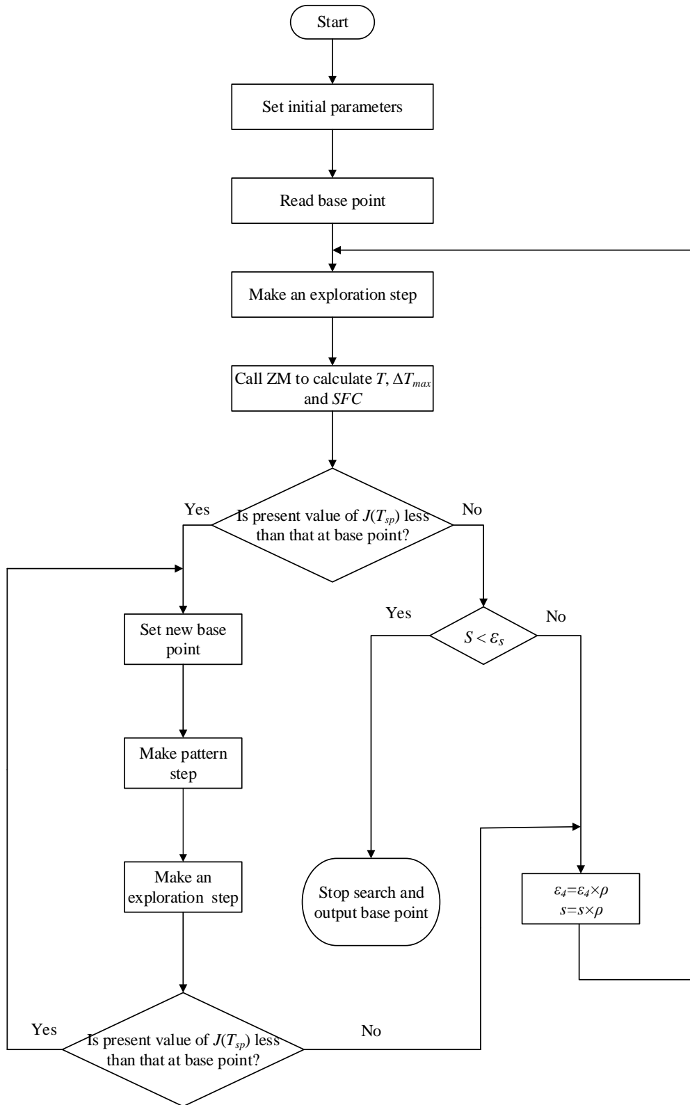
Figure 4. Flow chart of Hooke-Jeeves direct search algorithm (HJDSA) for seeking desired set-point temperatures.
