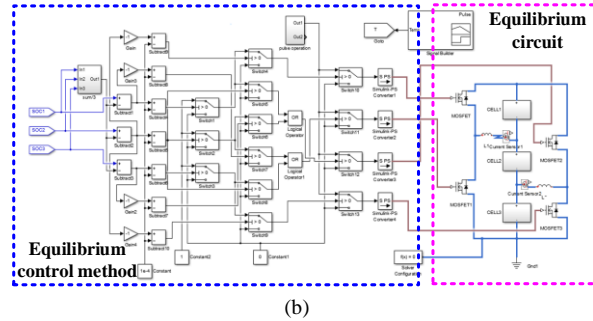
Fig.14 The simulation model in MATLAB-Simulink. (a) The equivalent circuit model of one battery cell; (b) The equalization model.
