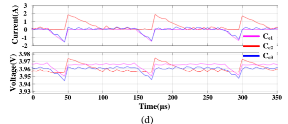
Fig.15 Simulation results of the proposed equalization process under the standing condition.(a) The change of SOC ( C_{e1}>C_{e2}>C_{e3} ); (b) The change of SOC ( C_{e2}>C_{e1}>C_{e3} ); (c) The change of SOC ( C_{e2}>C_{e3}>C_{e1} ); (d)The current and voltage of cells ( C_{e1}>C_{e2}>C_{e3} )
