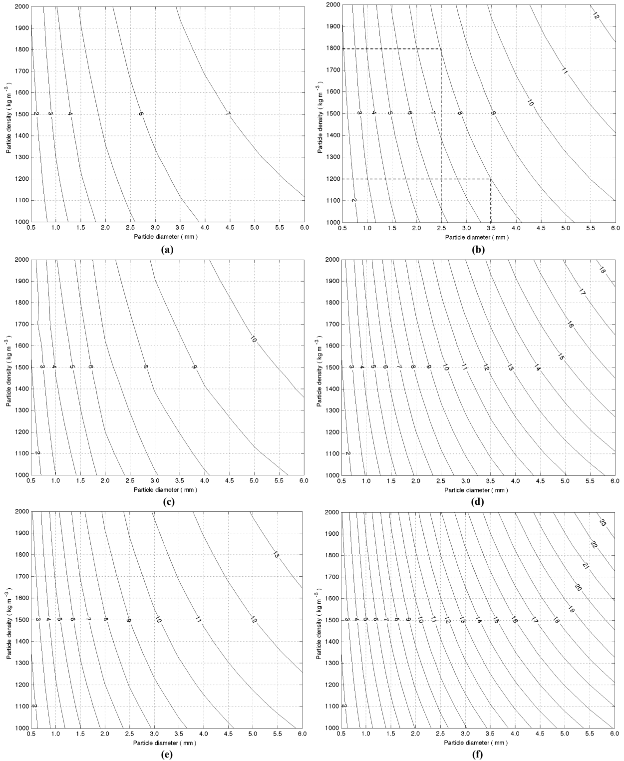
Figure 5. Contour plots used to determine landing distance of individual fertilizer particles based on particle diameter and particle density. Launch conditions are: h_0 = 1 m, and (a): \alpha_0 = 0^\circ , v_0 = 20 m s -1 , (b): \alpha_0 = 10^\circ , v_0 = 20 m s -1 , (c): \alpha_0 = 0^\circ , v_0 = 30 m s -1 , (d): \alpha_0 = 10^\circ , v_0 = 30 m s -1 , (e): \alpha_0 = 0^\circ , v_0 = 40 m s -1 , and (f): \alpha_0 = 10^\circ , v_0 = 40 m s -1 . In (b), dashed lines illustrate the example given in the text for two fertilizer materials with d = 2.5 mm and \rho_p = 1800 kg m -3 , and d = 3.5 mm and \rho_p = 1200 kg m -3 , respectively.
