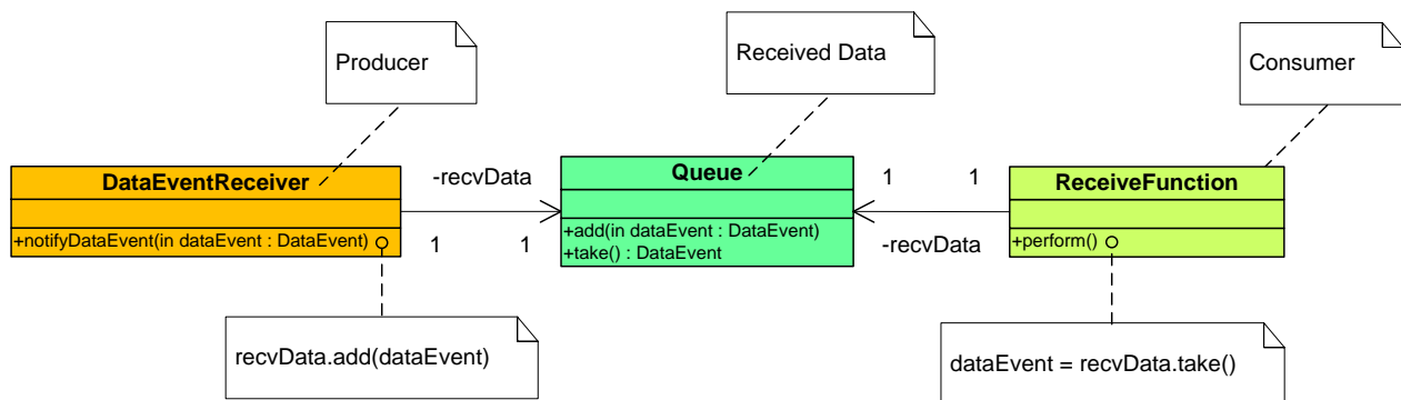
Fig. 10. Producer/Consumer Pattern.
