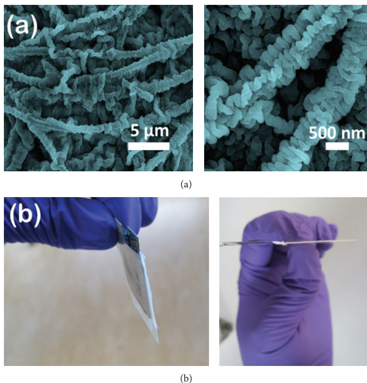
FIGURE 2: (a) Different morphology of MnO 2 with change in preparation conditions on CNFs. (b) Photos of as-assembled supercapacitor in (~2 mm thick) semiplane and its cross-sectional view.
