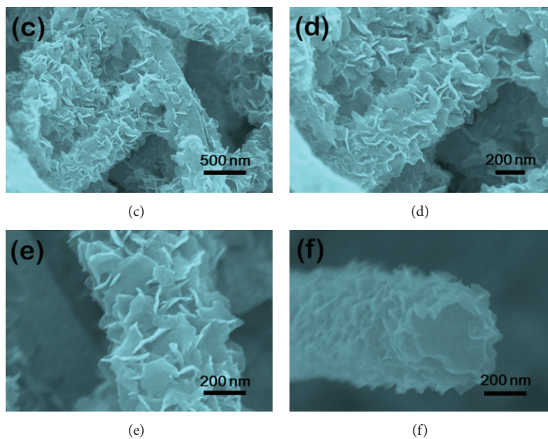
FIGURE 1: (a) Schematic of coating 2D \text{MnO}_2 nanosheets onto CNFs surfaces at room temperature. (b) XRD patterns of as prepared CNFs- \text{MnO}_2 crystal structures. (c)–(f) SEM images of CNF- \text{MnO}_2 mats with different magnifications.
