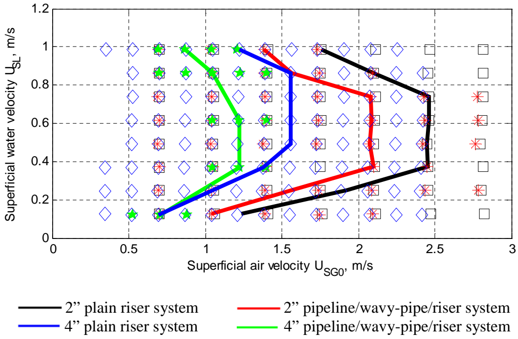
Fig. 6 Stability boundaries for the 2" and 4" plain riser and pipeline/wavy-pipe/riser systems
