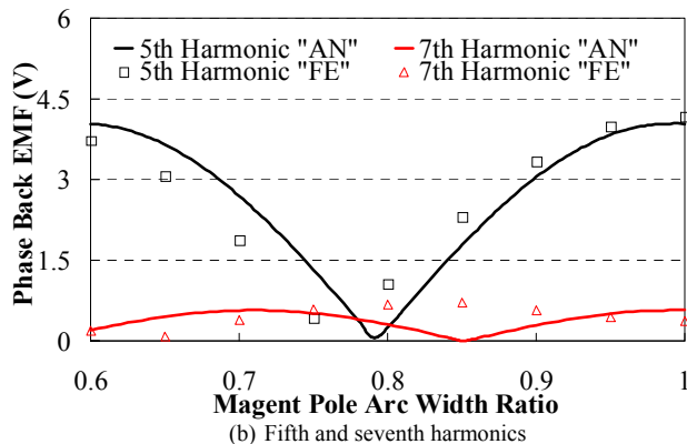
Fig. 5. Phase back EMF characteristics for different MPAW from analytical ("AN") and 2-D FEA ("FE") models.
