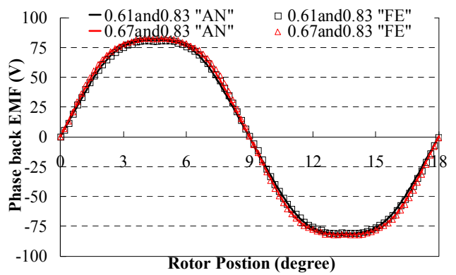
Fig. 14. Phase back EMF waveforms with the proposed axial pole pairs from analytical ("AN") and synthesized 2-D FEA ("FE") models.
