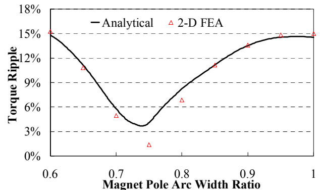
Fig. 7. Variation of torque ripple with MPAW at rated output torque.
