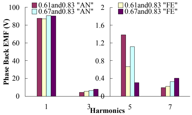
Fig. 15. Harmonic spectrum of the phase back EMF with the proposed axial pole pairs from analytical ("AN") and synthesized 2-D FEA ("FE") models.
