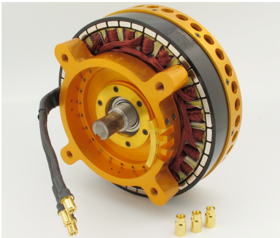
(b) Assembled prototype machine showing design for manufacturability Fig. 18. Prototype machine implemented and built with the 0.61/0.83 MPAW pole-pair for experimental validation
