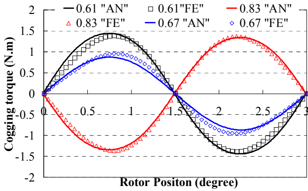
Fig. 11. Cogging torque waveforms for the machines with 0.61, 0.67, 0.83 MPAW predicted by analytical ("AN") and 2-D FEA ("FE") models.
