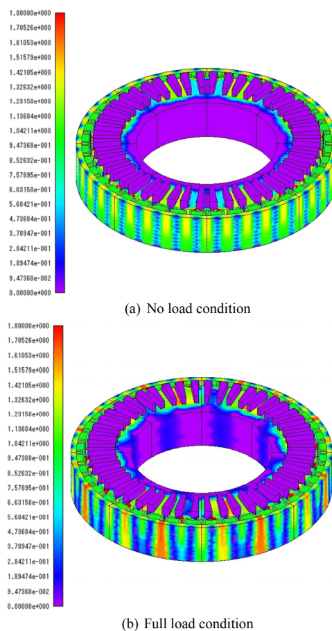
Fig. 17. Flux density distributions of the machine with the proposed axial pole
