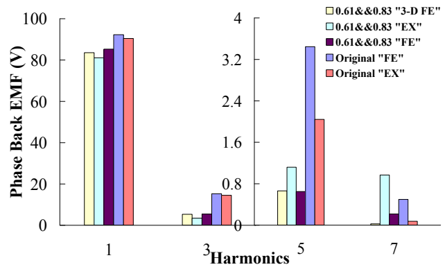
Fig. 21. Harmonic spectrum of the phase back EMF of the two prototypes from 2-D FEA ("FE"), 3-D FEA ("3-D FE"), and experiments ("EX").
