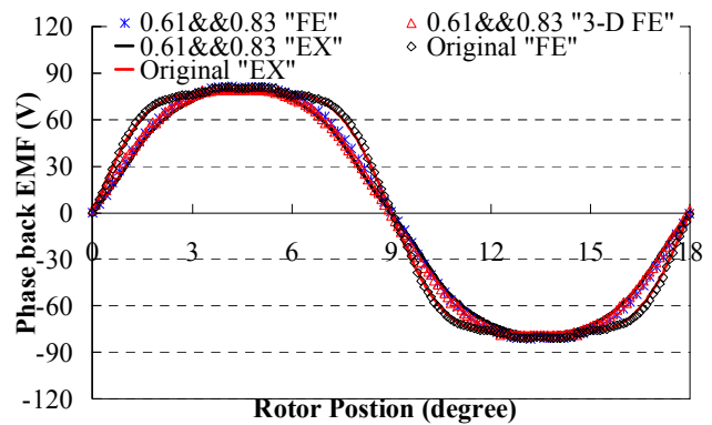
Fig. 20. Phase back EMF waveforms for the two prototypes from 2-D FEA ("FE"), 3-D FEA ("3-D FE"), and experiments ("EX").
