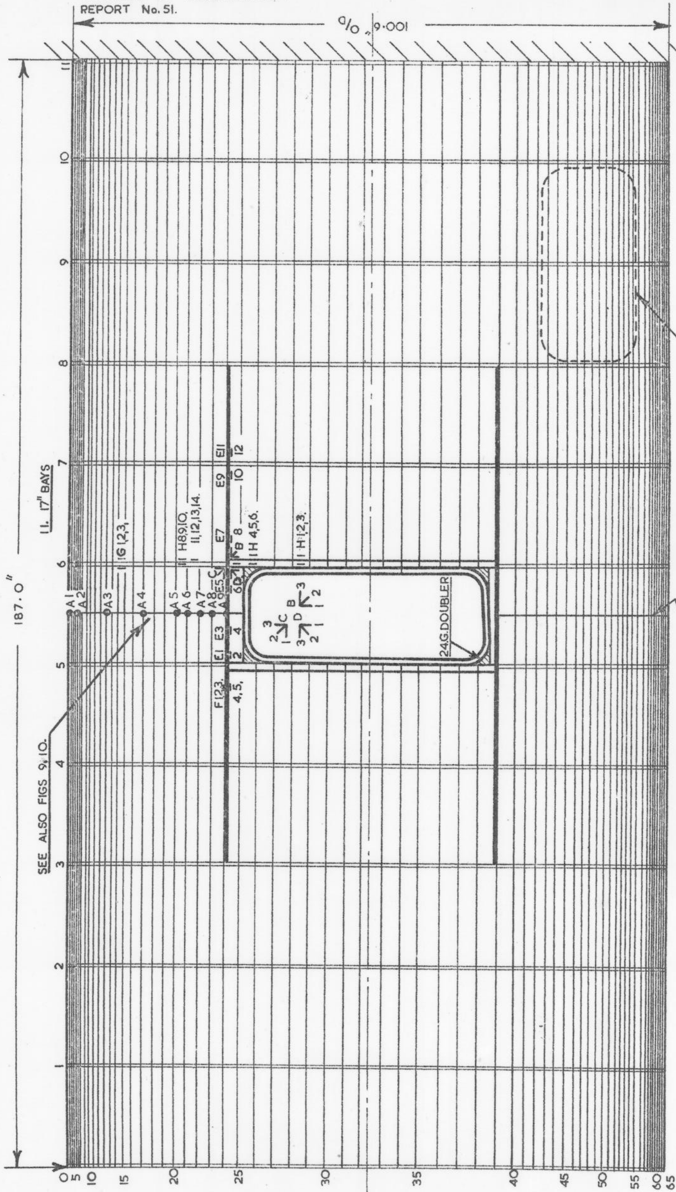
AS FIG. 10. LINE OF SKIN SHEAR GAUGES ARRANGEMENT OF STRAIN GAUGES.
