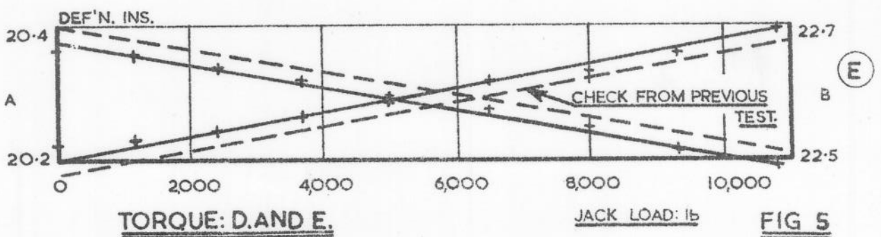
EXAMPLE OF: STRAIN GAUGE READING AND DEF'N — JACK LOAD
