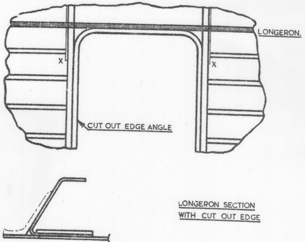
(b) SUGGESTED STRUCTURE NOT TO SCALE.
