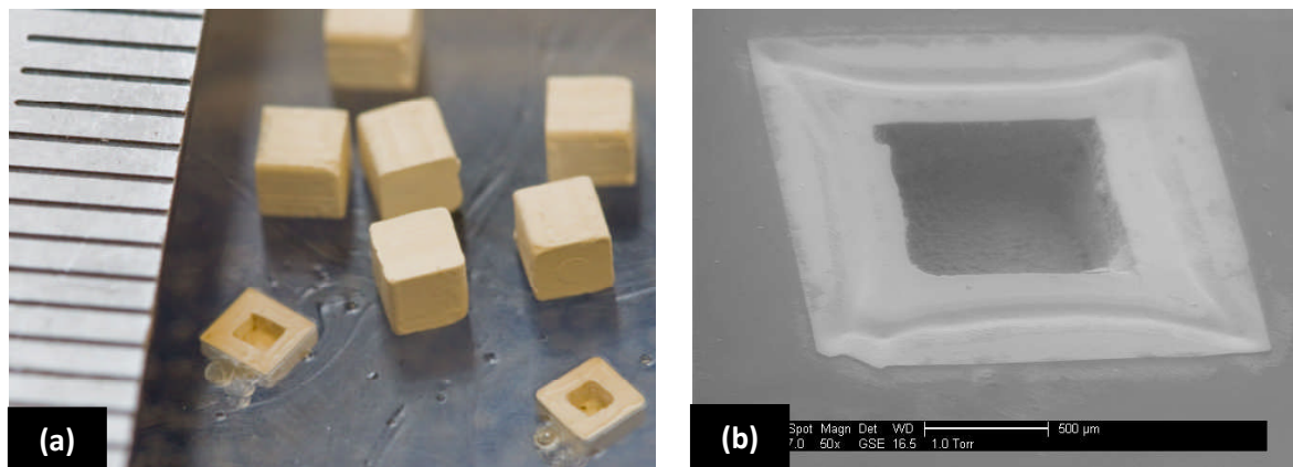
Fig. 4. a) An image of debinded components before sectioning and after sectioning while immersed in resin. b) An ESEM image of a sectioned brown component showing the hollow core.
