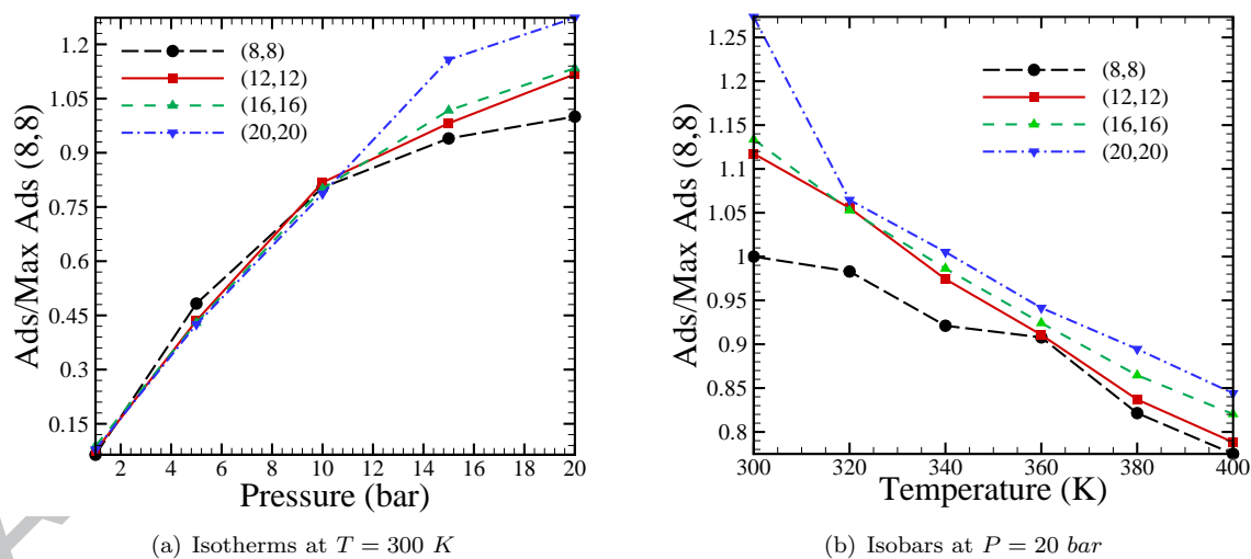
Figure 4: Adsorption isotherms and isobars for various nanotubes normalized by the case of (8, 8) nanotube at P = 20 bar and T = 300 K
