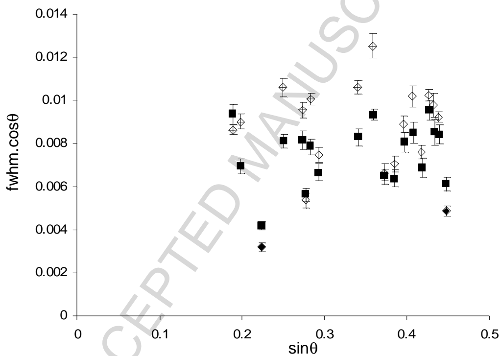
Fig. 4. Williamson–Hall plots indicating instrument corrected diffraction peak widths plotted for each unequivocal peak within the diffraction data. Data presented are unheated archaeological bone ( \diamond ), and contemporary bone heated to 600 °C ( \blacksquare ). Further, for the archaeological bone, widths corresponding to hk0 ( \diamond ) and 00l reflections ( \blacklozenge ) are indicated. Error bars are standard errors, ( n = 15 ).
