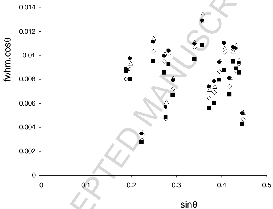
Fig. 5. Williamson–Hall plots indicating the instrument corrected diffraction peak widths plotted for each species with the archaeological series. Data presented are ( \diamond ) cow, ( \blacksquare ) human, ( \triangle ) pig, and undifferentiated ( \bullet ) sheep/goat.
