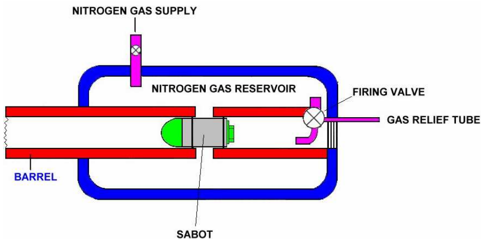
Figure 3 schematic of the compressed gas powered gun
