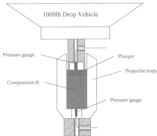
Figure Schematic of the NSW setback simulator
