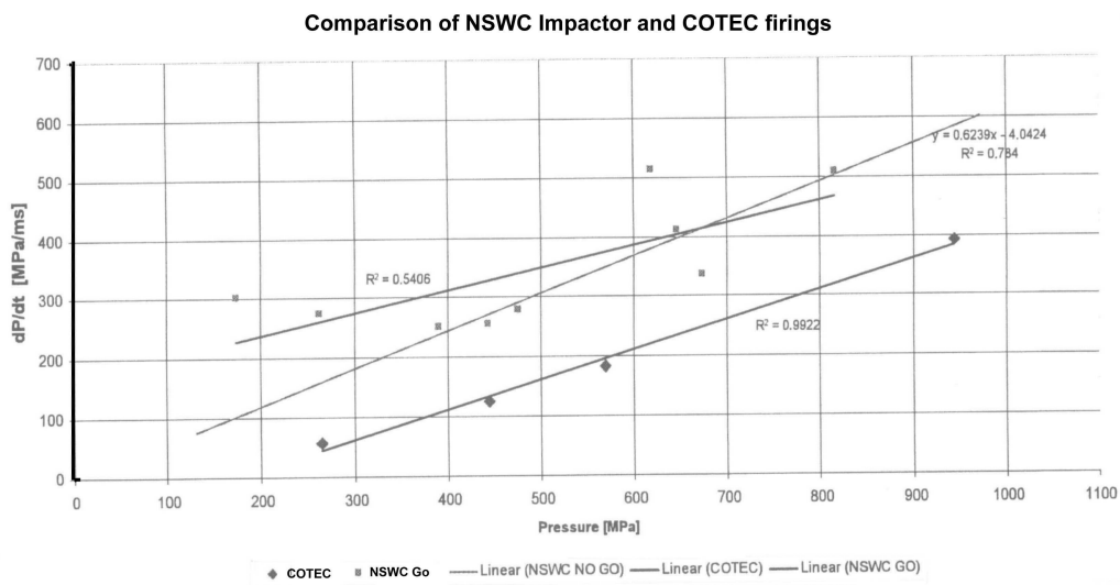
Figure 10 Comparison of NSWC and COTEC results for Composition B
