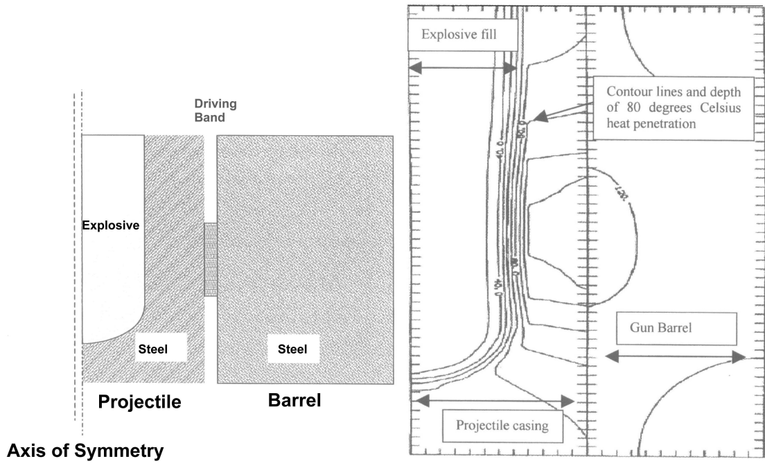
Figure 4 Area of contact between projectile and Barrel and the depth contour lines for the 80°C heat penetration as a function of time
