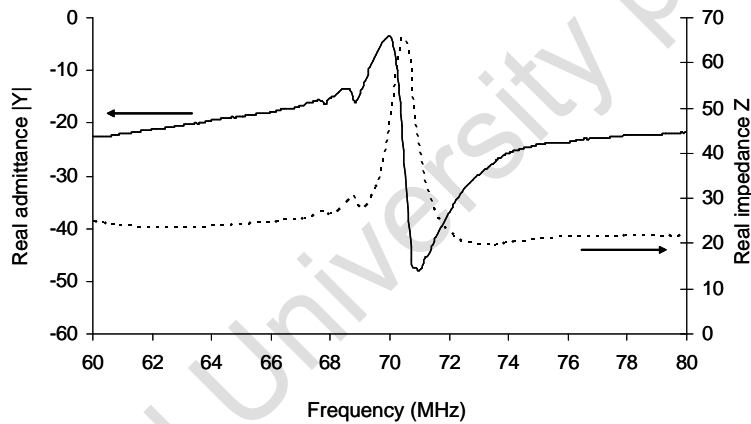
Fig. 6. Response for a 24µm thick device structure
