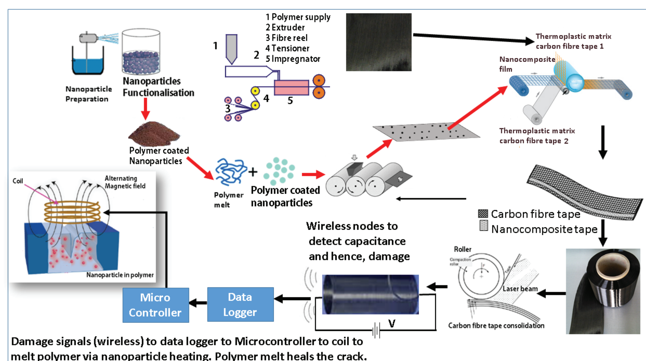
Figure 1: Schematic showing concept of bulk sandwich tapes with processing steps to prepare tubular structure and its intelligent healing process using magnetic flux stimuli.
