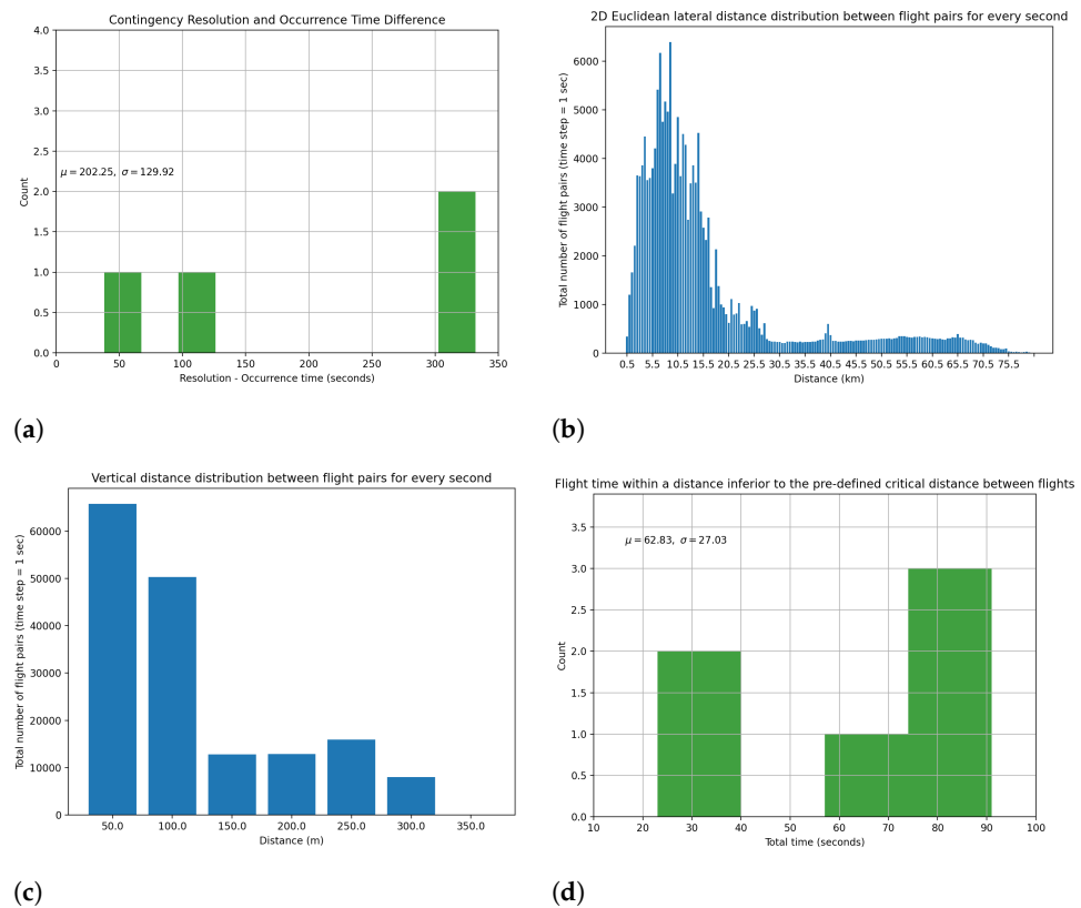
Figure 12. Analysis on contingency resolution process and collision possibility analysis. (a) Contingency resolution time. (b) Pairwise lateral distance. (c) Pairwise vertical distance. (d) Flight duration within crucial distance.
