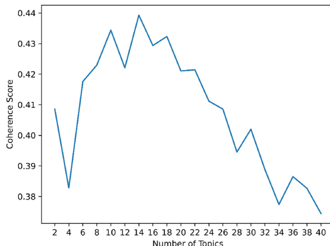
Fig. 1. Coherence scores plot.
