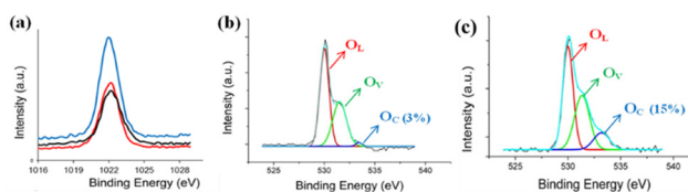
Fig. 6 (a) Zn 2p XPS spectra peaks of ZNWs and ZNLs, (b) O 1s XPS spectra of ZNWs, and (c) O 1s XPS spectra of ZNLs.
