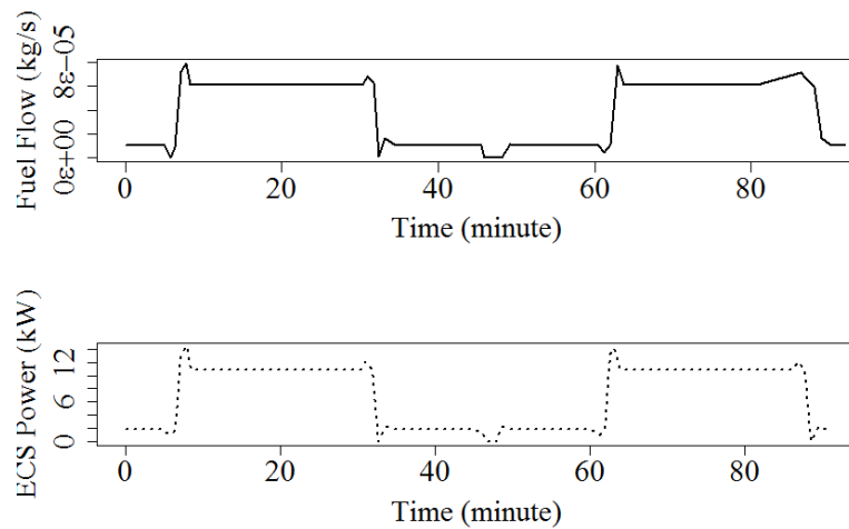
Fig. 7 Environmental Control System fuel flow (Baseline & Reference), and power demand (Conceptual)
