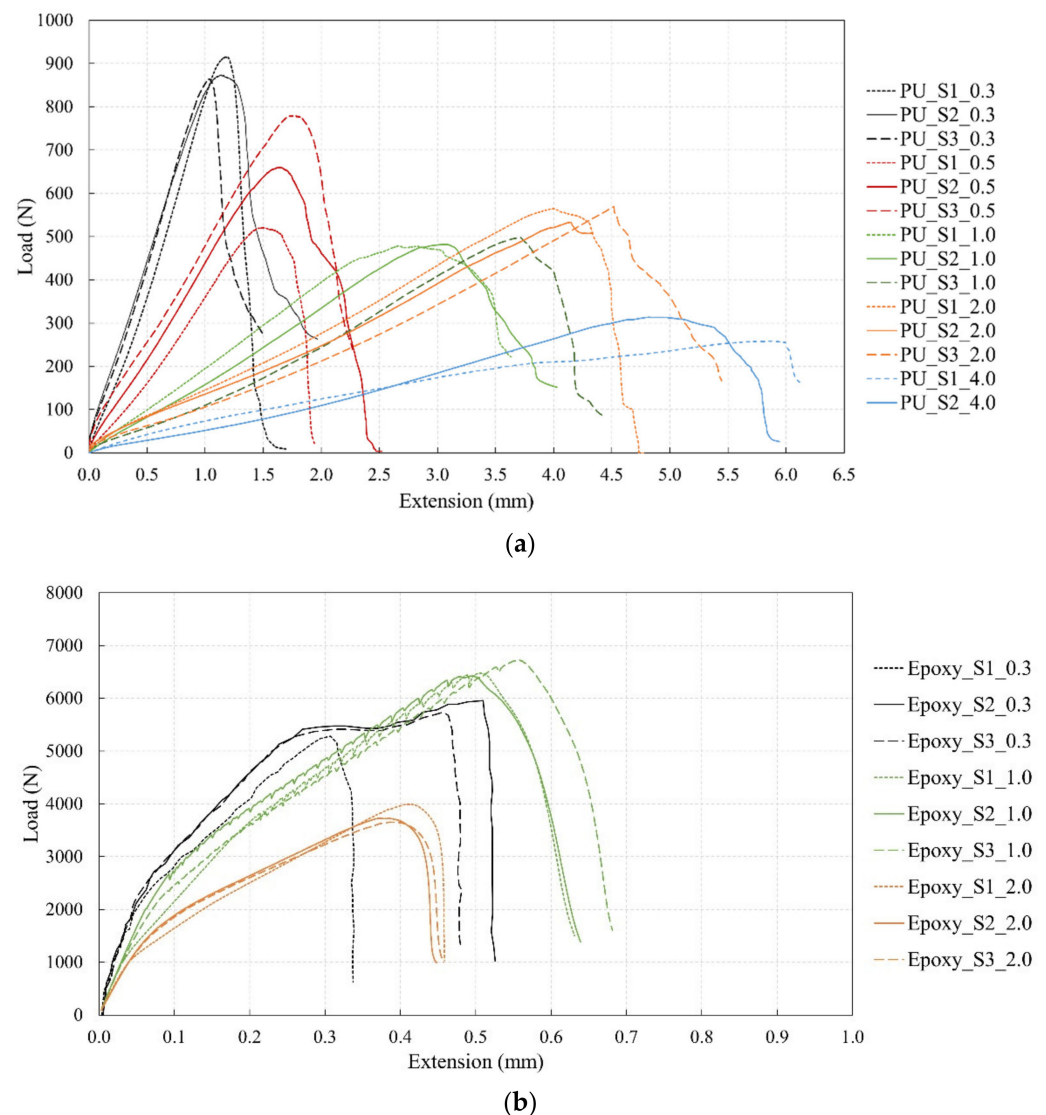
Figure A1. The load-extension curves of the adhesive bonded joints using (a) polyurethane adhesive (PU) with different adhesive thicknesses (0.3, 0.5, 1.0, 2.0 and 4.0 mm) and (b) epoxy adhesive with different adhesive thicknesses (0.3, 1.0 and 2.0 mm).
