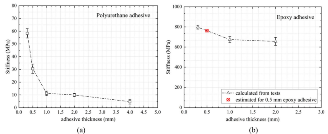
Figure 8. Stiffness of the joints vs. bond gap using (a) polyurethane and (b) epoxy adhesives. The point marked with a red cross in (b) is an interpolation of the joint stiffness for the 0.5 mm epoxy adhesive.
