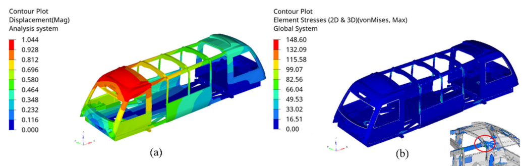
Figure 9. (a) Displacement and (b) stress distribution of the vehicle under torsional loading case using 0.3 mm epoxy adhesive (scale factor = 5). Units are in mm and MPa.
