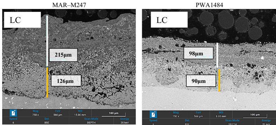
Fig. 3 Backscattered images of cross sections through alloy MAR-M247 and PWA 1484 samples covered with deposits ( 80\% \text{Na}_2\text{SO}_4 – 20\% \text{K}_2\text{SO}_4 ) exposed to air + 300 vppm SO x gaseous atmosphere gas within long cyclic test conditions for 560 h between 700–900 °C
