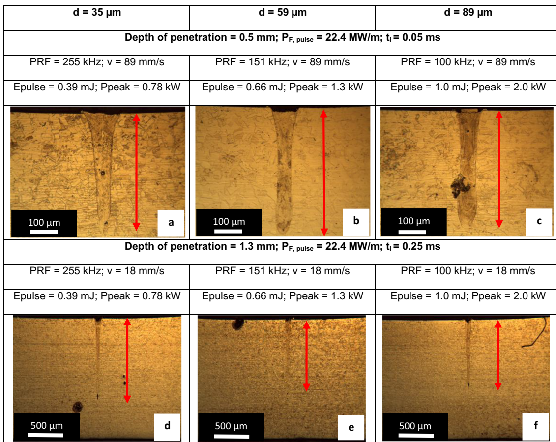
Fig. 13 Constant combinations of pulse power factor of 22.4 MW/m and interaction times of 0.05 ms and 0.25 ms for different beam diameters of 35, 59 and 89 \mu\text{m}
