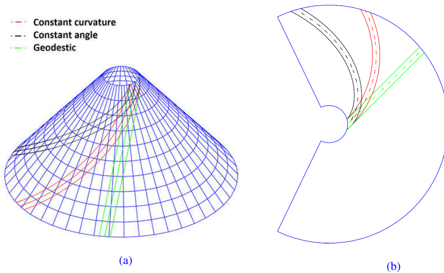
Figure 14: Comparison of the definition of the fibre angle trajectory based on the geodesic path with those based on the constant angle and constant curvature paths. a) Paths on the 3-D conical shell, b) Paths on the flattened cone. Adapted with permission from Blom [70].
