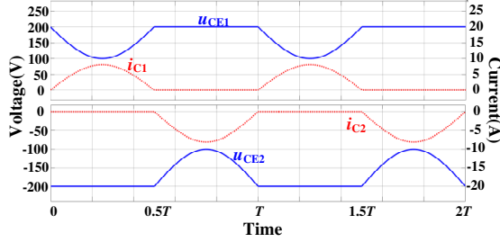
Fig. 4. The voltage and current waveforms on T 1 and T 2 under the Normal power supply mode.
