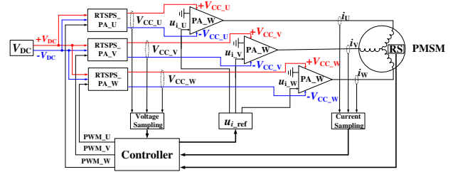
Fig. 17. The PMSM drive topology based on PAs and the RTSPSs.
