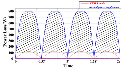
Fig. 7. Losses comparison of PA between two modes.
