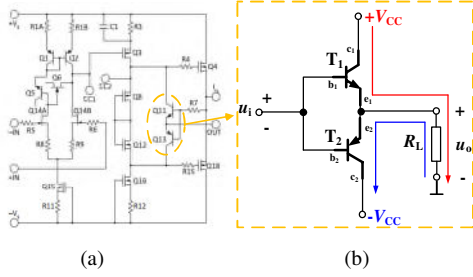
Fig. 1. OCL power amplifier circuit. (a) Internal structure. (b) Simplified structure.
