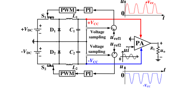
Fig. 10. Circuit structure of the proposed RTSPSs.
