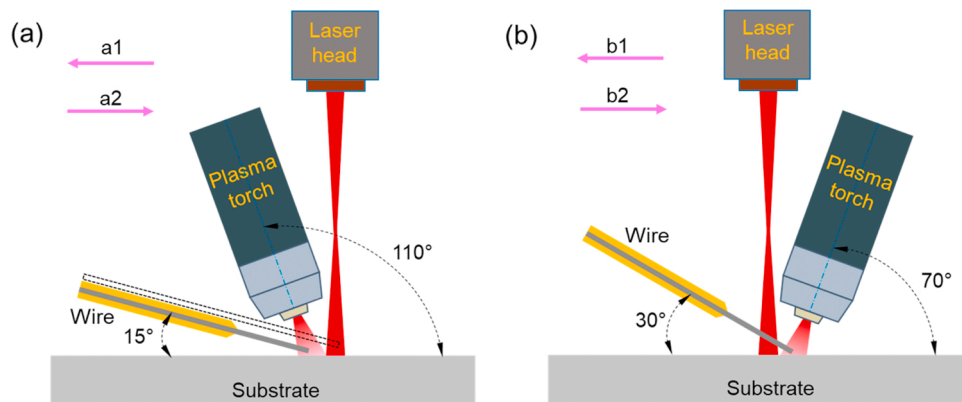
Fig. 2. Different configurations and travel directions (indicated by pink arrows) used: (a) the wire is first irradiated by the PTA, and (b) the wire is first irradiated by the laser.
