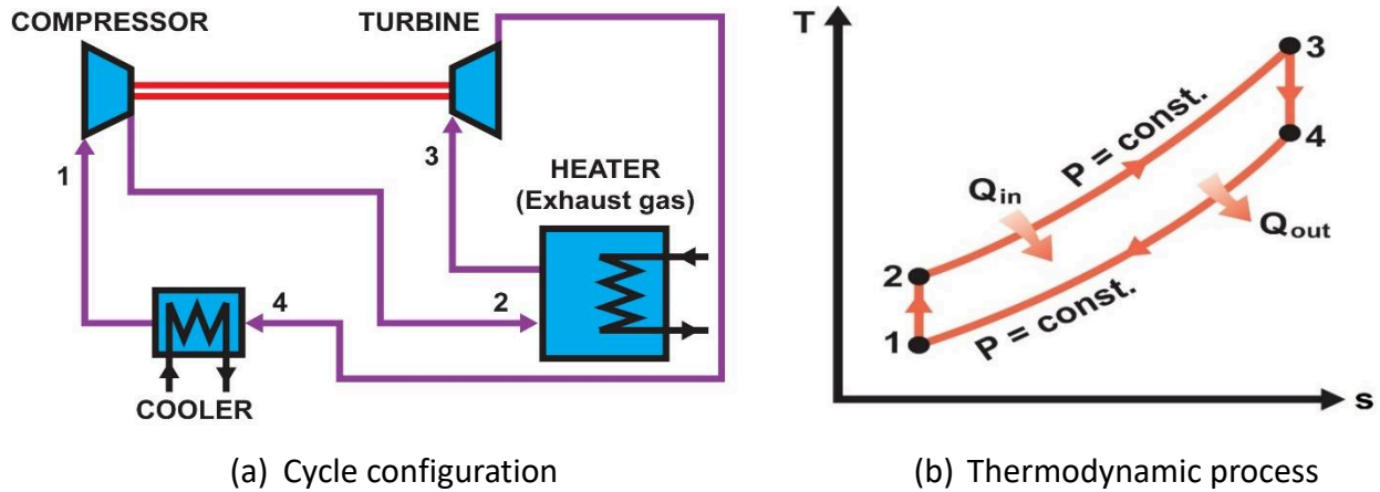
Fig. 1 Schematic and T-s diagram of the Basic Brayton cycle
