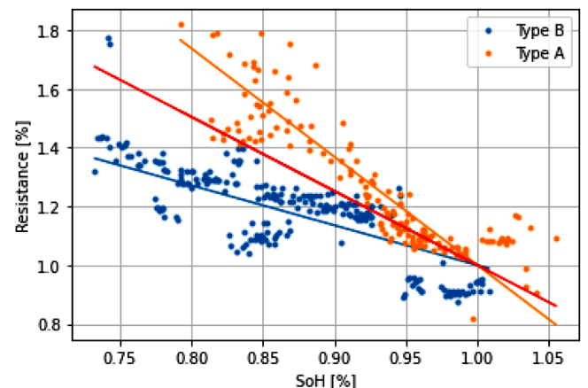
Figure 3. DC Resistance in dependency of the SoH.
