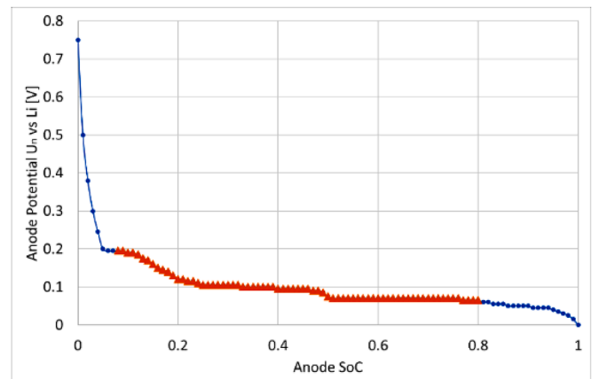
Figure 8. Anode Potential Curve [52].
