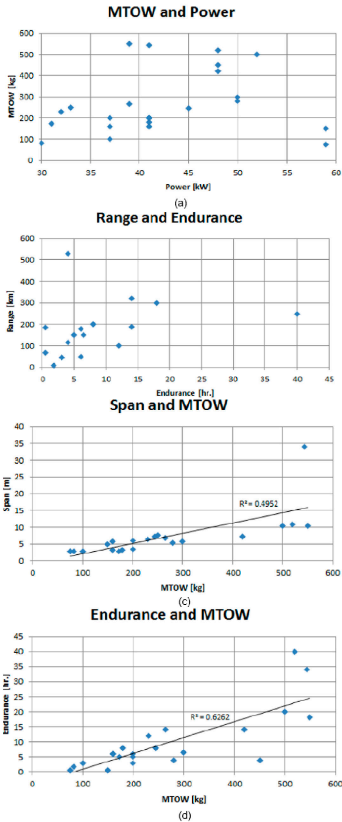
Figure 2. Performance trend of existing unmanned aerial vehicles (UAVs) (a) Maximum take-off weight against power (b) flight range against endurance (c) Span against maximum take-off weight (d) endurance against maximum take-off weight [1,12].
