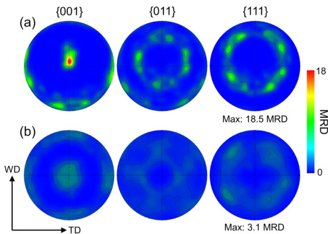
Fig. 3. ‘Before and after’ pole figures showing the bulk textures of the WAAM tensile specimen (a) grip (coarse columnar \beta structure, Fig. 2), and (b) the whole recrystallized region, following rapid re-heating, near the fracture surface (Fig. 4).
