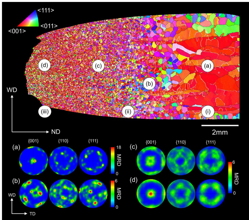
Fig. 4. \beta -reconstructed EBSD orientation map of the recrystallized microstructure at the centre plane of the deformed and rapidly heated sample, sectioned back from the WAAM tensile specimen fracture surface. The pole figures (a-d) show the micro-textures at the positions marked on the tensile specimen with corresponding strains of \sim 1 , 15, 26, and 37%, respectively.
