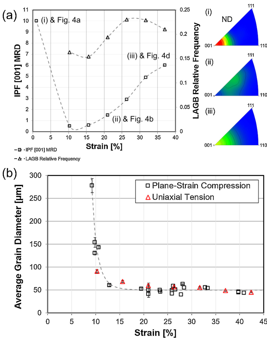
Fig. 5. Statistical EBSD data from along the sample gauge length of the rapidly heat treated sample shown in Fig. 4, as a function of the local strain showing; (a) strength of the \langle 001 \rangle_{\beta} // ND pole in MRD and the relative frequency of LAGBs (compared to HAGBs), (b) the average recrystallized \beta -grain sizes compared to previous results for the plane strain compression study conducted in ref. [12]. In (a) the IPFs (i-iii) correspond to the pole figures in Fig. 4a,b,d, respectively, and show the texture change with position.
