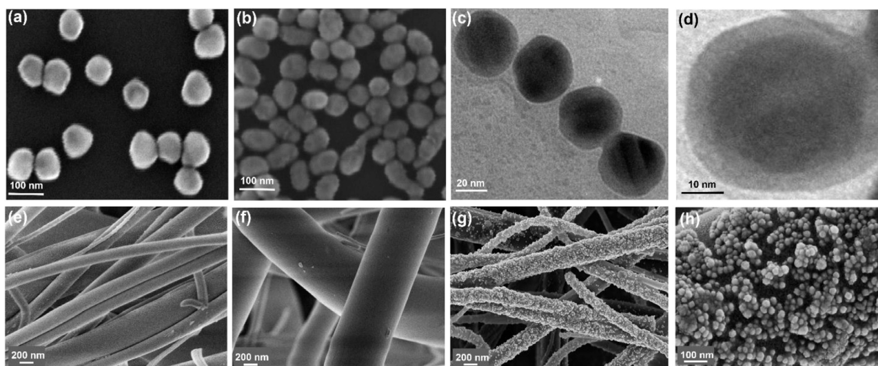
Fig. 2. Evaluation and characterization of Au@Ag assembled on the glass nanofibrous paper substrate: (a) Field emission scanning electron microscopy (FE-SEM) image of prepared Au nanoparticles; (b) FE-SEM image of prepared Au@Ag core-shell nanoparticles; (c) Low-magnification high-resolution transmission electron microscopy (HR-TEM) image of Au@Ag; (d) High-magnification HR-TEM images of Au@Ag; (e) Low-magnification FE-SEM image of glass nanofibrous paper; (f) High-magnification FE-SEM image of the glass nanofibrous paper substrate; (g) Low-magnification FE-SEM image of Au@Ag-pLL assembled on the glass nanofibrous paper substrate; (h) High-magnification FE-SEM image of Au@Ag-pLL assembled on the glass nanofibrous paper substrate.
