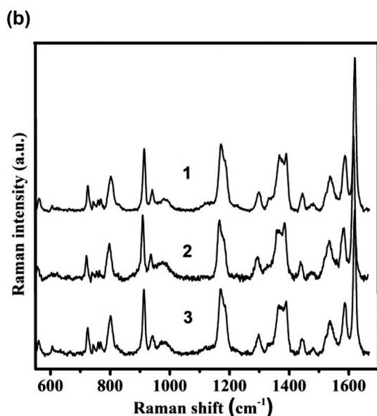
Fig. 3. (a) SERS spectra of CV (100 nM) acquired from 8 different SERS substrates within a SERS array, showing a high degree of reproducibility; (b) SERS spectra ( \lambda_{\text{ex}} = 785 \text{ nm} ) of CV (100 nM) acquired from a freshly prepared Au@Ag-pLL-GNFP SERS substrate (No. 3) and from a substrate prepared one month (No. 2) and two months (No. 1) earlier, showing good long-term stability of the nanofibrous paper-Au@Ag assembly.
