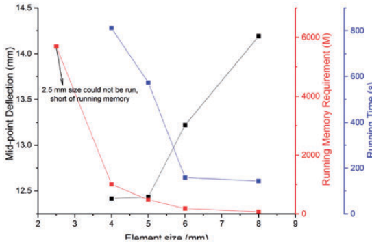
Figure 1. Mesh convergence test detailing relationship between element size, maximum deflection and memory requirement.
