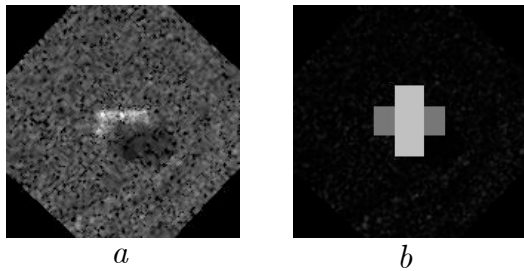
Fig. 3: Location of the areas whose summed intensities are used to compute the vertical ratio and tackle 90^\circ errors. a Image of a rotated and centred target in the MSTAR dataset at 0^\circ . b Location in the MSTAR of the rectangles used to compute the vertical ratio.
