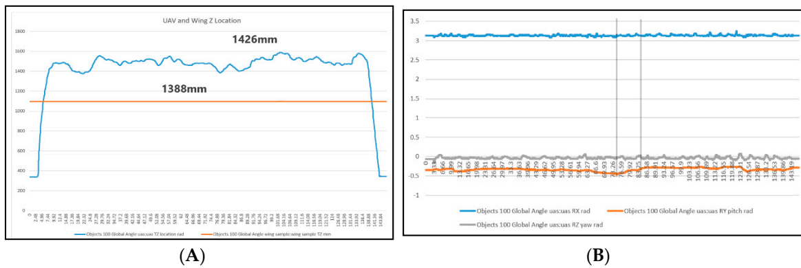
Figure 21. (A) The z -axis shows the flight envelope: 1426 \text{ mm} - 1388 \text{ mm} = 38 \text{ mm} . (B) Graph demonstrating the stability of the UAV in flight. This was measured by the roll along the x -axis, pitch along the y -axis, and yaw along the z -axis.
