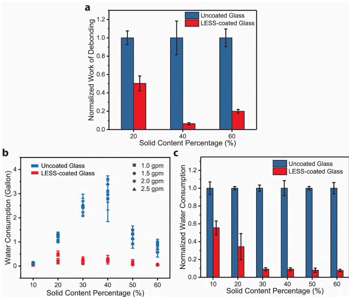
Figure 4. Work of adhesion and water consumption characterizations. a, Work of debonding of synthetic feces of varying solid contents on uncoated bare glass and LESS-coated glass. The data is normalized by the work of debonding of the synthetic feces on uncoated glass. b, Water consumption measurements on uncoated and LESS-coated glass under different flow rates after being impacted by ~5 grams of synthetic feces with different solid content percentage. Error bars represent standard deviations of four independent measurements. c, Cleaning water consumption performance of different surfaces after synthetic feces impact. The data is normalized by the
