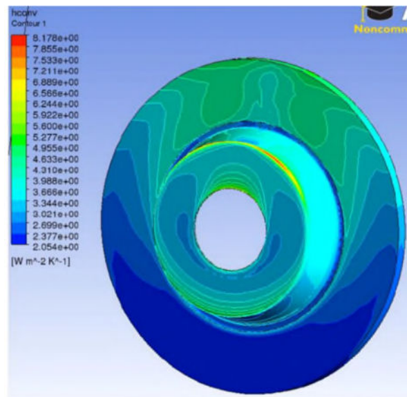
Figure 15 Predicted convective heat transfer coefficient distribution for solid disc
