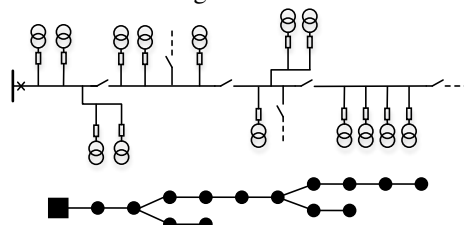
Fig. 1. Topology characterization of feeders
