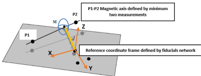
Fig. 4. The pre-alignment metrology defined as: spatial location (with uncertainty) of the magnetic axis (defined by minimum two 3D coordinates P1-P2) with respect to each assembly local coordinate frame (defined by minimum 3 fiducial spheres at the centre of one them).
