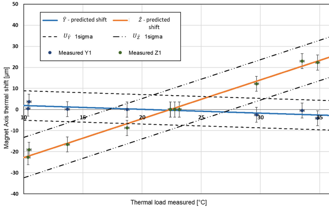
Fig. 15. Magnet axis location empirical model shift prediction and associated 1σ uncertainty of the prediction VS validation measurement samples and their standard uncertainty.
