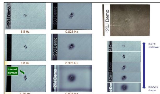
Figure 8: Sample 20 J Demo, Reflection front face, PPT. The damage is visible on the front face, how, it's clear that the damage is much worse subsurface and spreads further than the impacted area [5].
