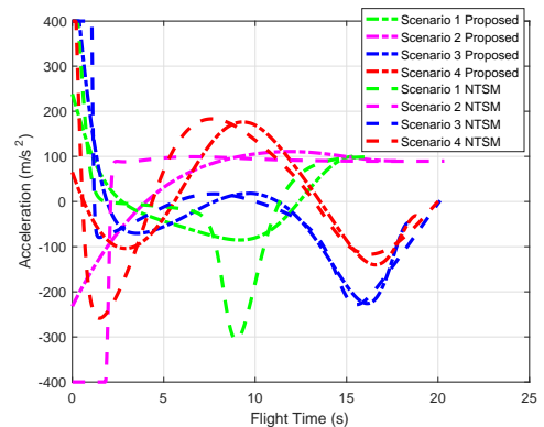
Fig. 6. Acceleration command.
