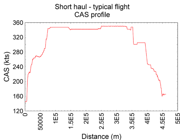
Fig. 6 London to Amsterdam typical flight: speed profile
