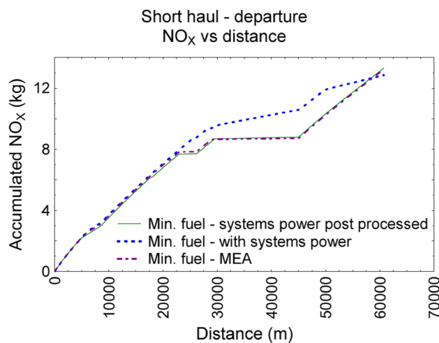
Fig. 14 Total NO x emissions vs distance—departure phase
