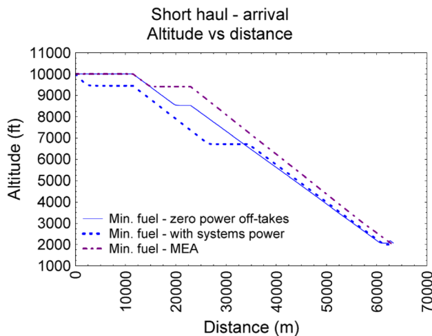
Fig. 22 Altitude vs distance—arrival, short haul
