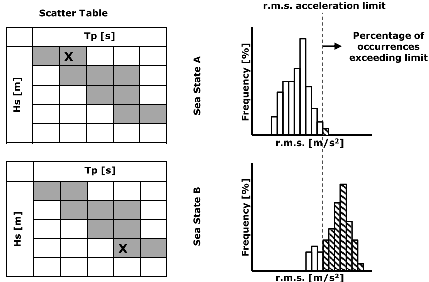
Fig. 9. Sea state dependent workability index.
