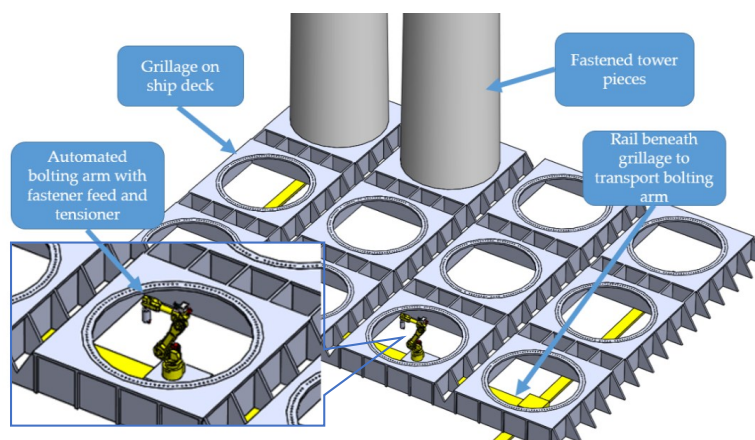
Figure 2. Automated bolted seafastening, concept illustration.
