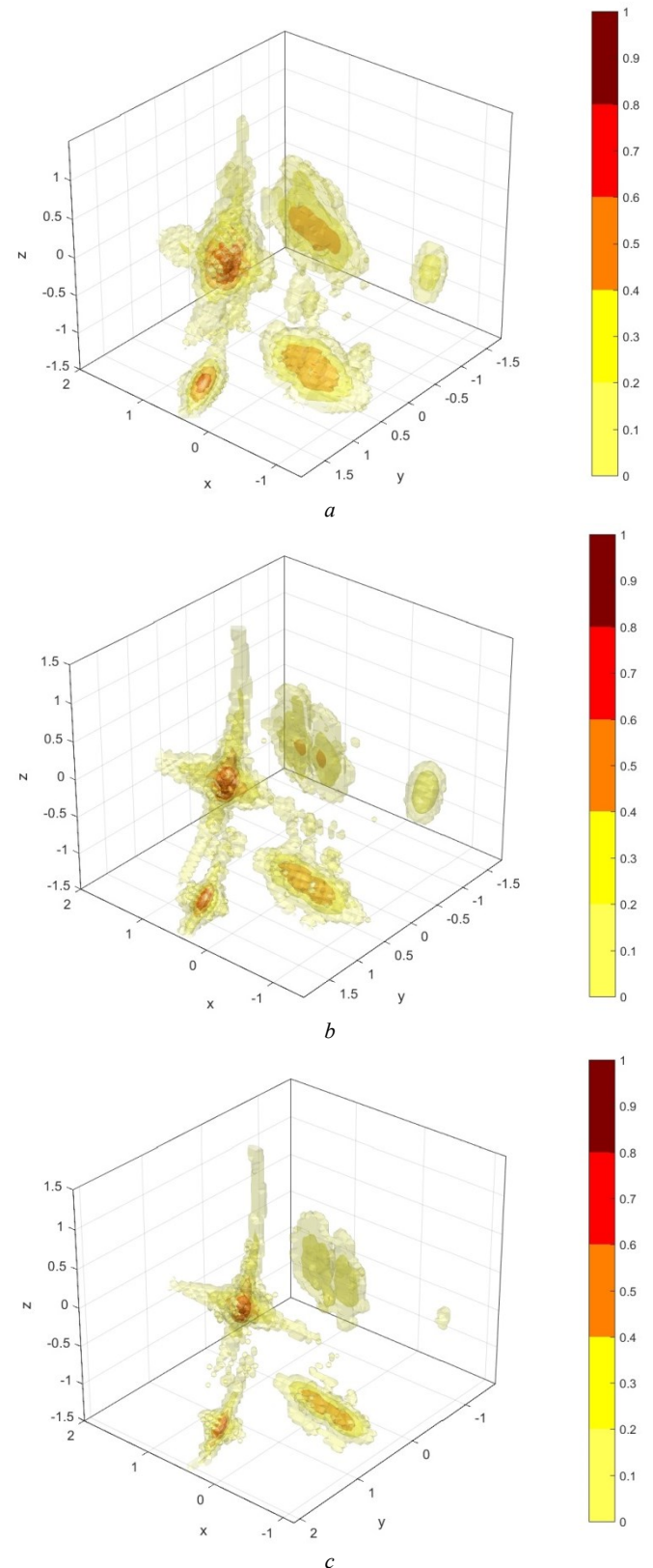
Fig. 4 Representations of a 3D LF SAR volumetric through-wall dataset, composed of partially transparent iso-brightness contour surfaces. The images were formed with three frequency sub-bands with 2GHz bandwidth, the sub-band centre frequencies being: a 2GHz, b 3GHz, c 4GHz.
