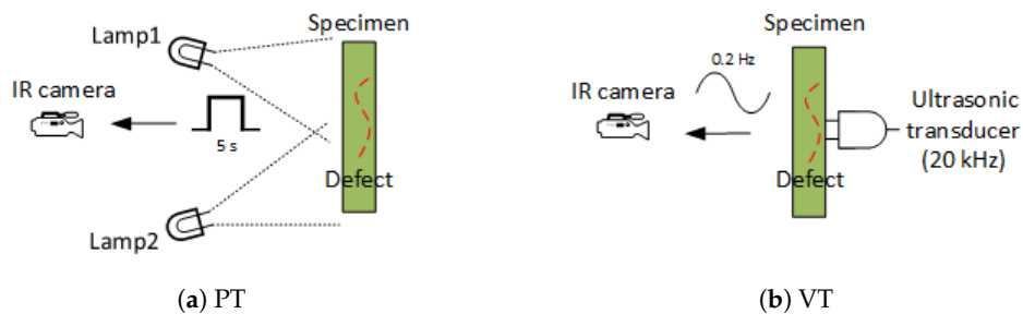
Figure 3. Schematic configurations.
