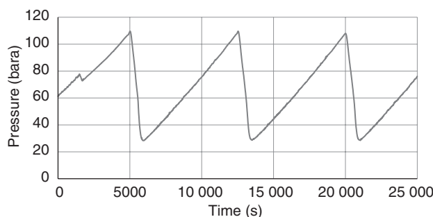
Fig 18: Severe slugging
