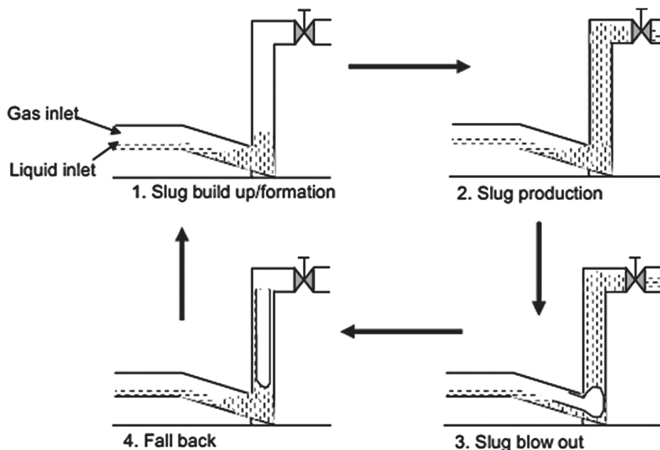
Fig 1: Different stages of severe slug (Ogazi, 2011)
