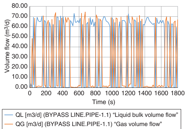
Fig 13: Gas and liquid flow at bypass
