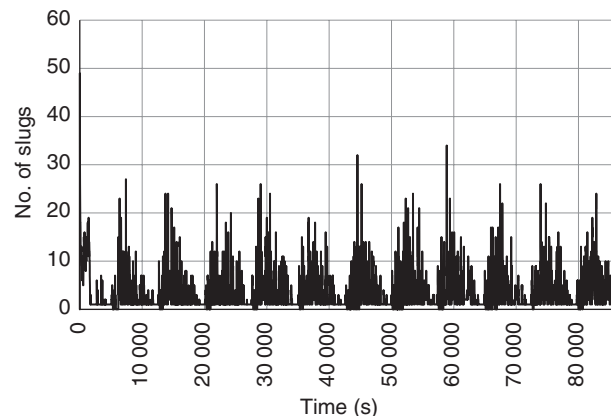
Fig 19: Number of slugs in the pipeline
