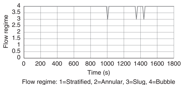
Fig 14: Flow regime at bypass
