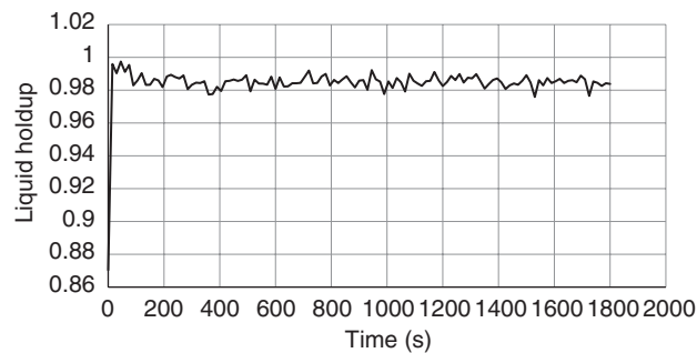
Fig 11: Liquid hold-up at riser base
