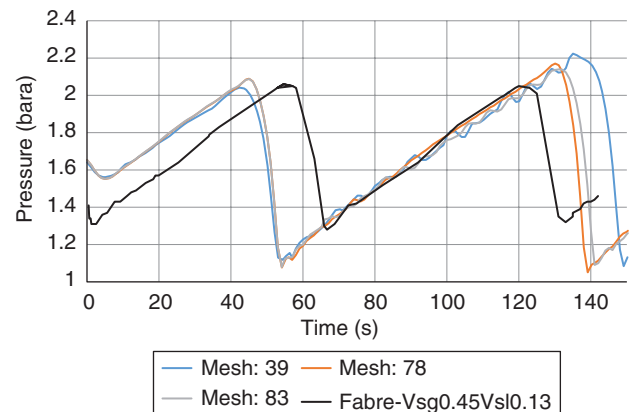
Fig 9: Mesh convergence of numerical model with literature data
