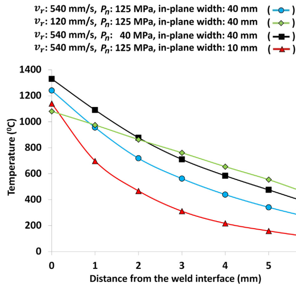
Fig. 10. Thermal profiles in Ti-6Al-4V linear friction welds showing the effects of the rubbing velocity, v_r , pressure, P_n , and in-plane width. These profiles were obtained from FEA [13,14].
